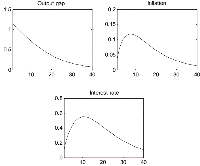
Figure 2: Impulse response analysis of an exogenous shock to output
